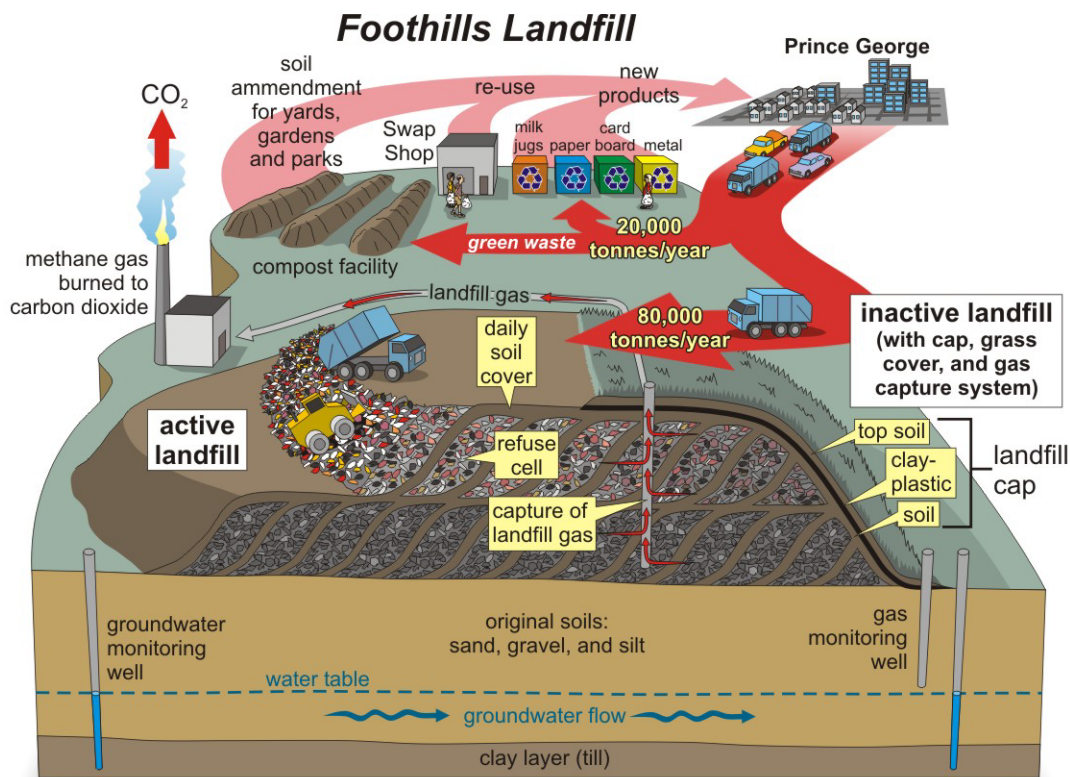
Figure 21: Schematic illustration of the Foothills landfill showing recycling, reuse, composting, landfill, and capture of landfill gases and groundwater effluents.
